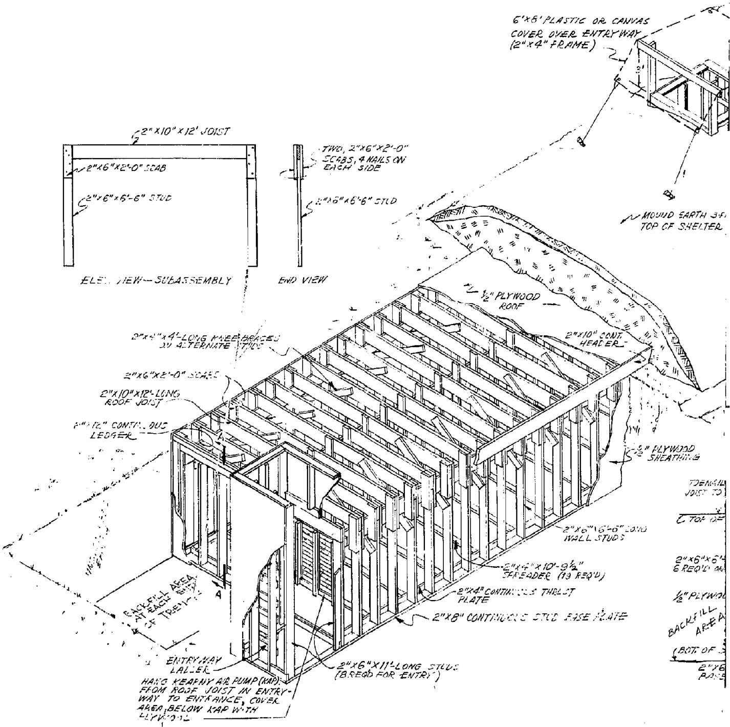
Fig. A-7.1. Rigid Frame Underground, Pictorial View.
